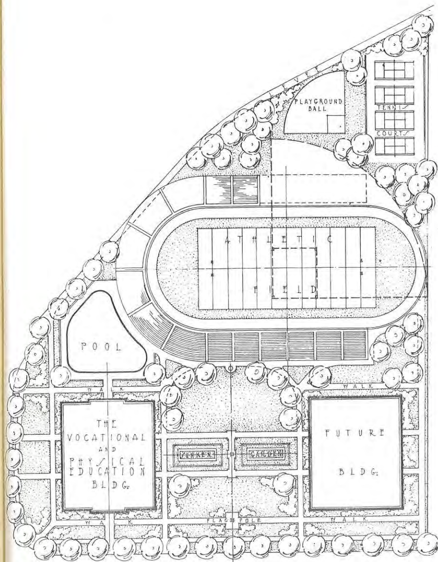
ATHLETIC PLANT LAYOUT, MUNCIE HIGH SCHOOL.
